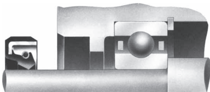
FIG. 10: Housing recess with locating flange.
