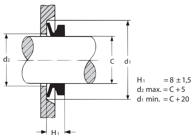
Dimensions, fitted
